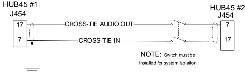
Figure 2 – Dual HUB45 Interface
