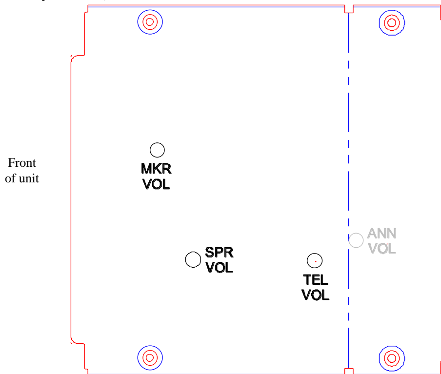
Figure 2-5- PMA8000B Adjustments, top cover
