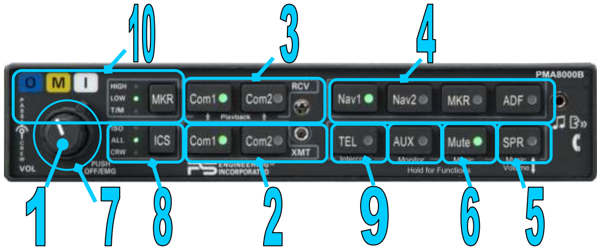
Figure 3-1 PMA8000B Operating Controls
