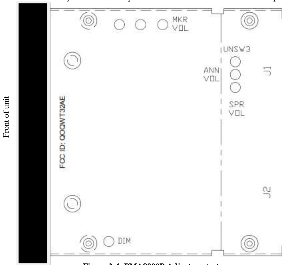
Figure 2-4- PMA8000B Adjustments, top cover
