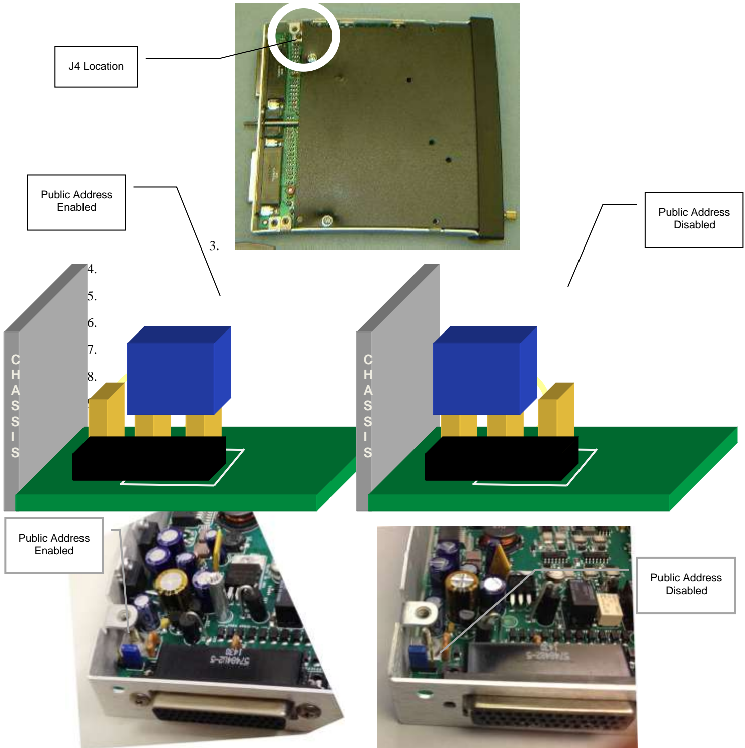
Figure 2-3 Jumper Location
