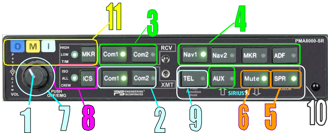
Figure 3-2 PMA8000-SR Operating controls
