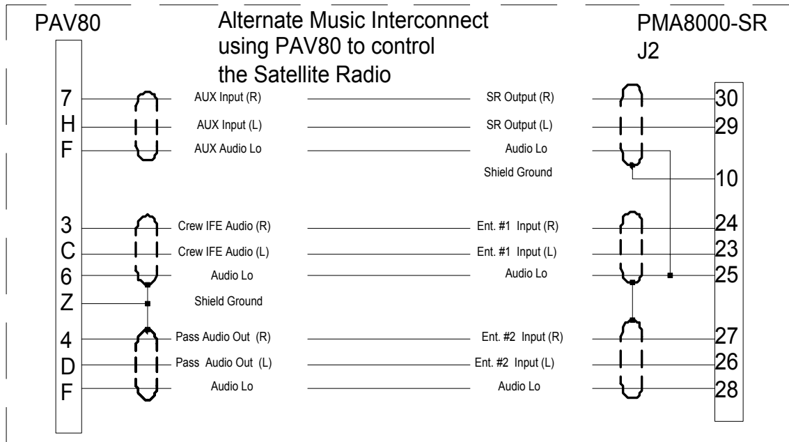
Figure 2-4 PMA8000-SR using PAV80 as control
