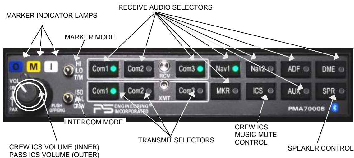
Figure 3-1 PMA7000BT controls
