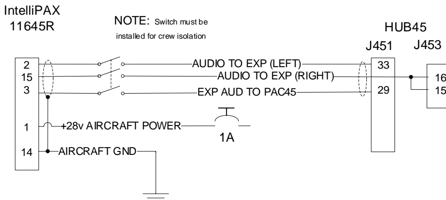
Figure 1 PAC45 system Interface
